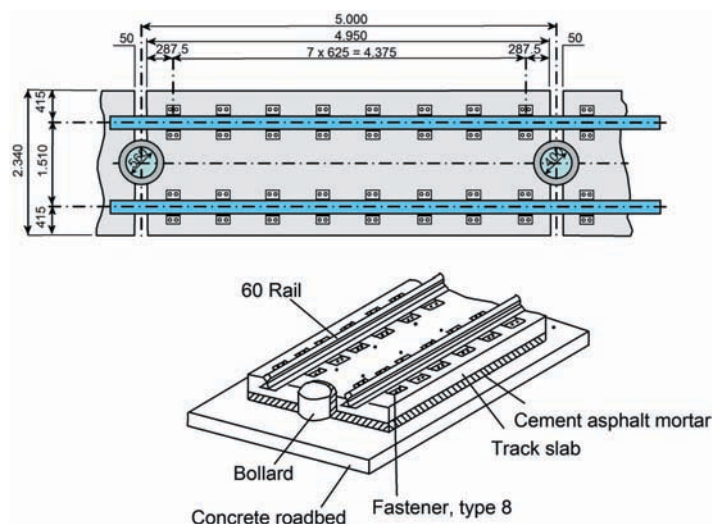
Fig. 1: Shinkansen slab track
