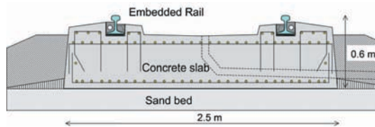
Fig. 5: Embedded rail track near Best (NL)
