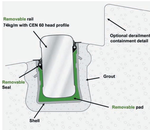
Fig. 7: Balfour Beatty embedded rail
